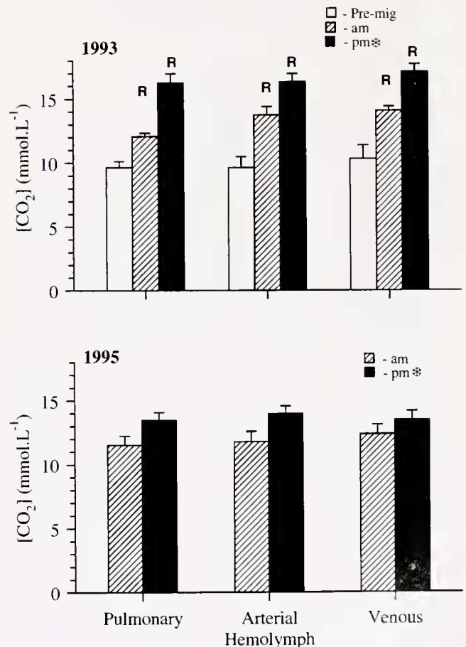
Figure 5. Carbon dioxide content ( [CO_2] , mmol \cdot l ^{-1} ) in the pulmonary, arterial, and venous haemolymph of Gecarcoidea natalis during two migration seasons, 1993 (top panel) and 1995 (bottom panel). Morning and afternoon groups were sampled during both migration seasons ( n = 5 in 1993; n = 9 in 1995). Top panel (1993 season) also includes measurements of [CO_2] in crabs 1 week prior to the start of the migration (pre-mig n = 12 ). The * symbol next to the legend indicates a significant difference between the AM and the PM groups. The "R" denotes a significant difference of a sample group from the crabs at rest—that is, from the resident pre-mig crabs.
